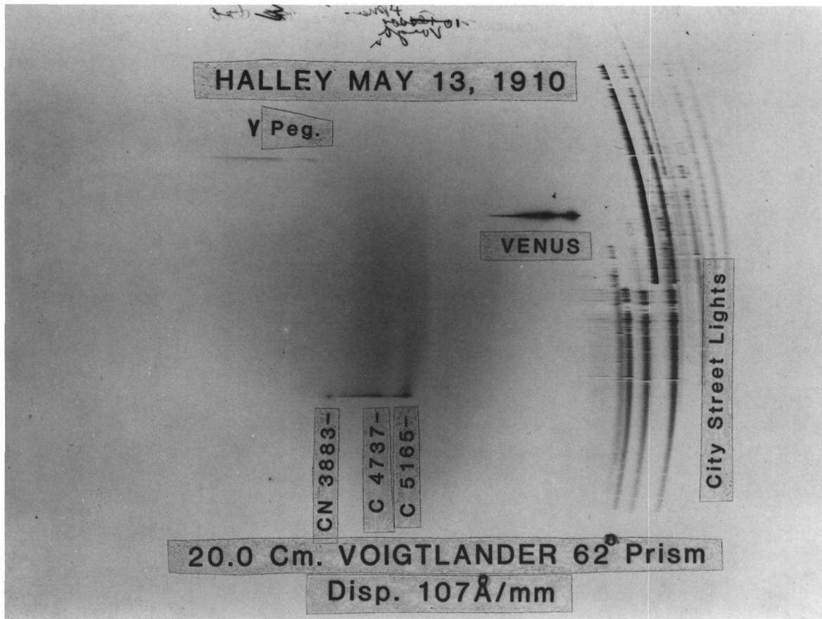
Figure 9. Objective prism spectrogram of Comet Halley obtained on May 13, 1910.
